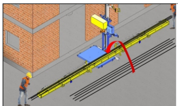
Loading Rebar
