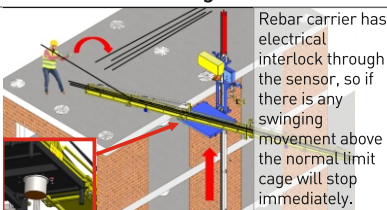
Unloading Rebar
