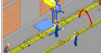
Rebar Attachment
