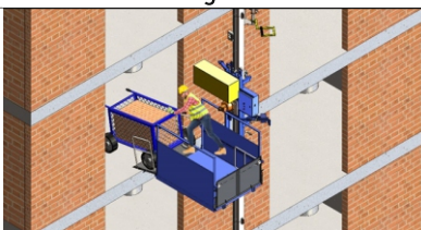
Unloading Bricks Carrier
