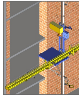
Cage with Rebar Carrying Attachment
